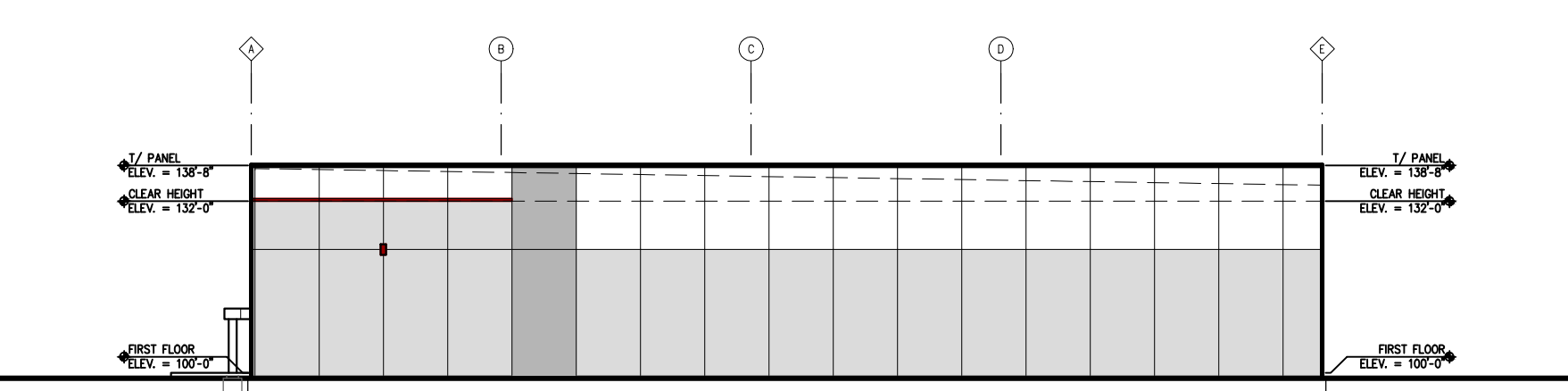
WEST ELEVATION
